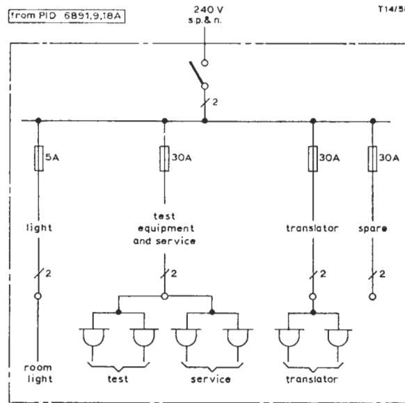
Fig. 1 Power Distribution Box BX3/3: Circuit
