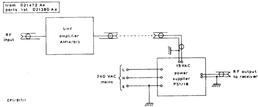
Fig. 1 Block Diagram of the EP1/517
