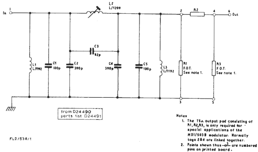
Fig. 1. Circuit of the FL2/536
