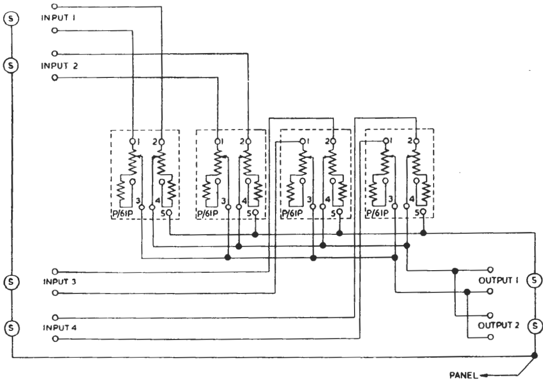
Fig. 13.6. Circuit MX/18
