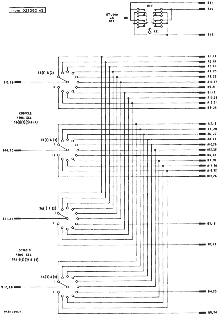
Fig. 1. Circuit of the PA8/290
