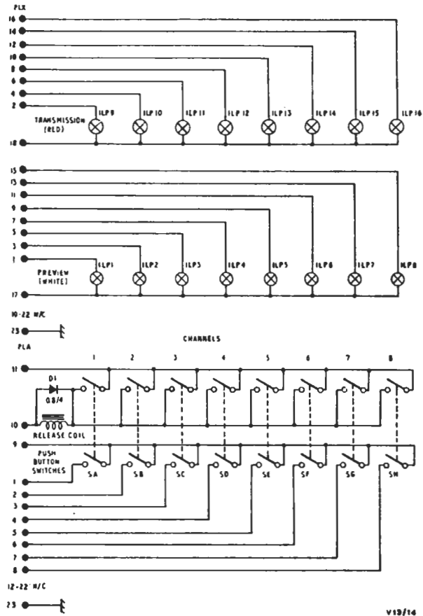
Fig. 11.1 Circuit of the PA8/511
