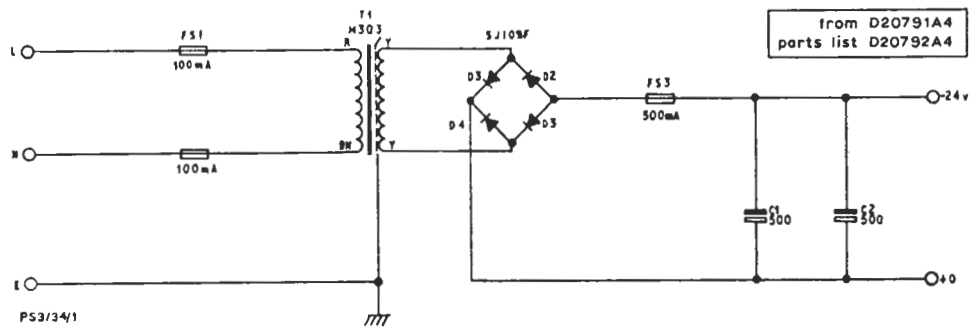
Fig. 1. Circuit of the PS3/34
