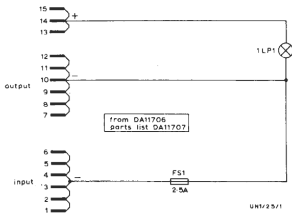
Fig. 1 Fuse and Indicator Unit UN1/25
