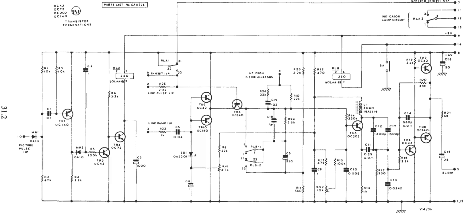
Fig. 31.2 Circuit of the UNI/531
