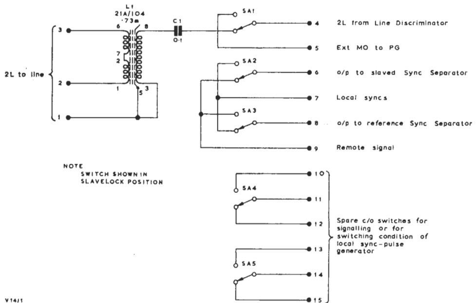
Fig. 15.1 Circuit of the UN9/515
